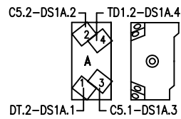
MACHINE (DS1) REMOTE/OFF/MANUAL
